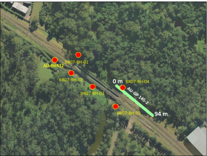
Seismic Refraction data limits
