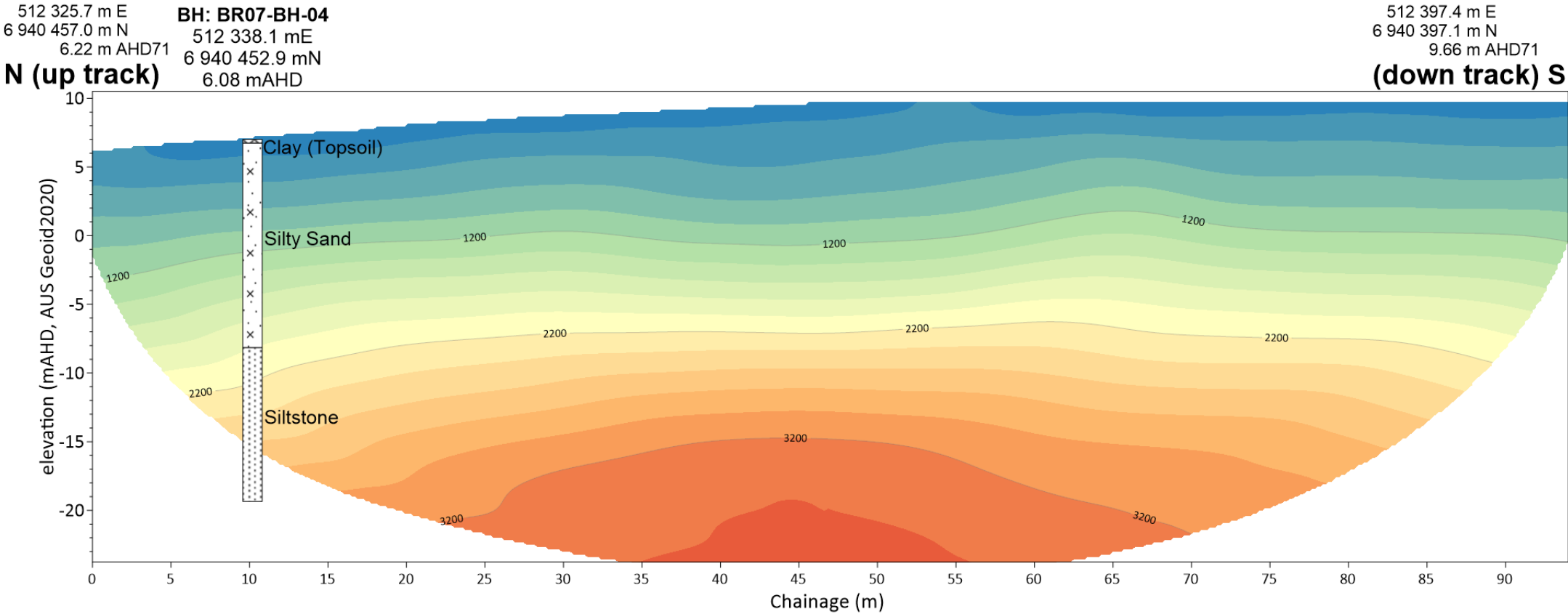
Seismic Line SR AU-GP 145-2
